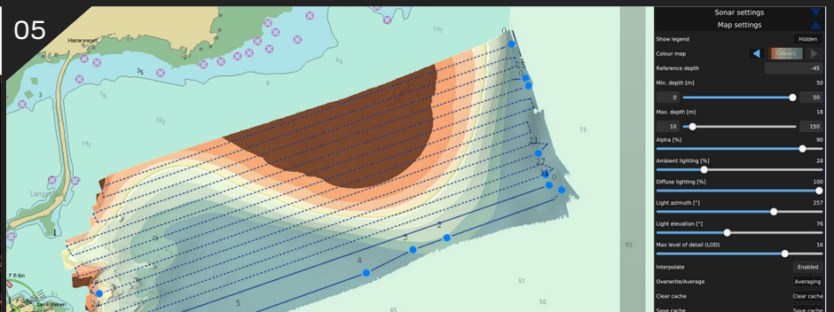
Bathymetry
